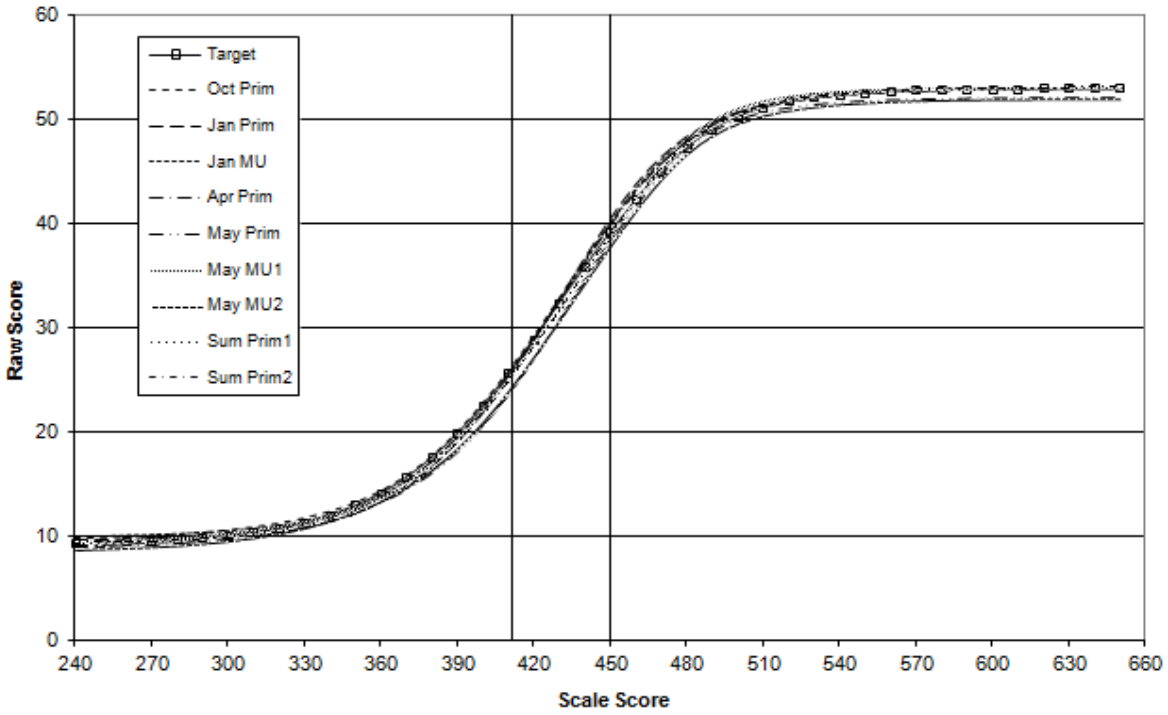
Figure 2.1 Test Characteristic Curves for the MD HSA 2012 Algebra Forms
