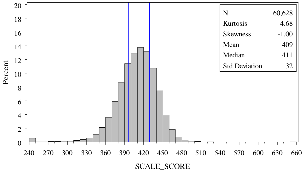
Figure 6.3 Histogram of Total Scale Scores for MD HSA May 2012 English
