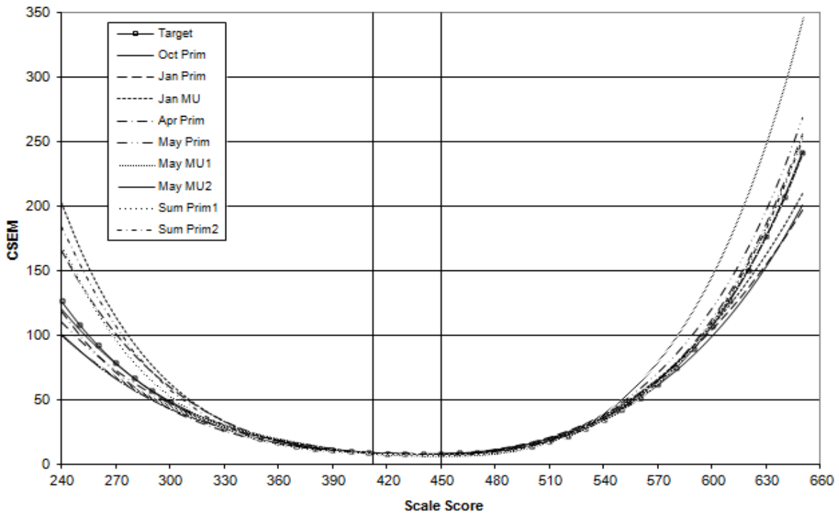
Figure 2.2 Conditional Standard Error of Measurement for the MD HSA 2012 Algebra Forms
