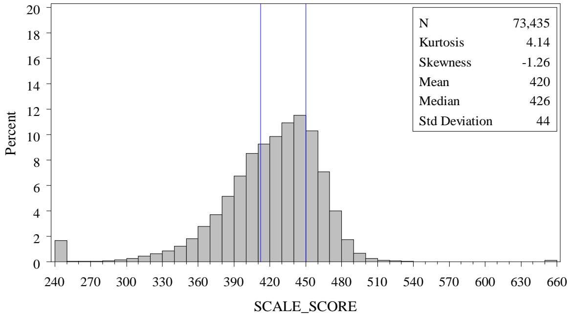
Figure 6.1 Histogram of Total Scale Scores for MD HSA May 2012 Algebra
