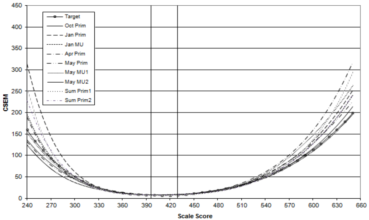
Figure 2.6 Conditional Standard Error of Measurement for the MD HSA 2012 English Forms
