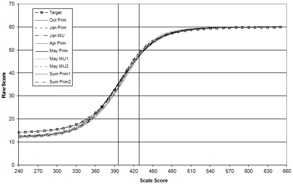
Figure 2.5 Test Characteristic Curves for the MD HSA 2012 English Forms
