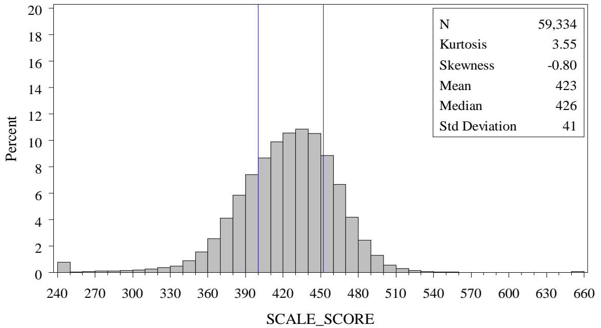
Figure 6.2 Histogram of Total Scale Scores for MD HSA May 2012 Biology
