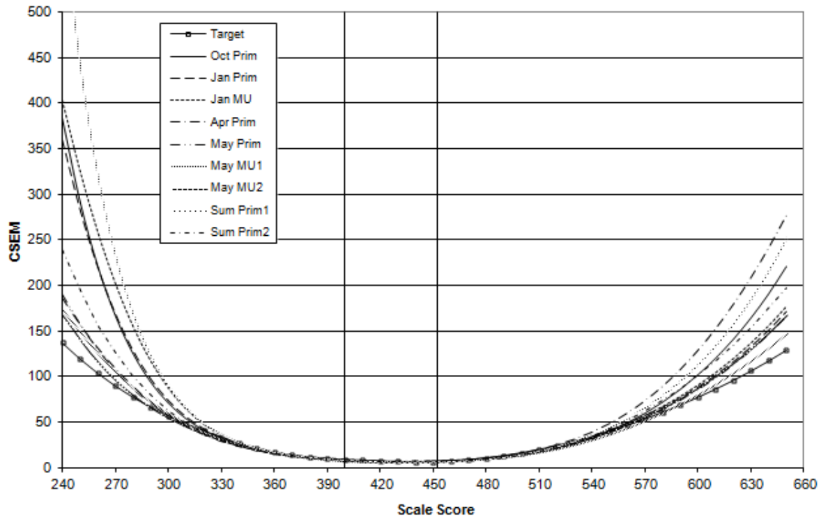
Figure 2.4 Conditional Standard Error Measurement for the MD HSA 2012 Biology Form
